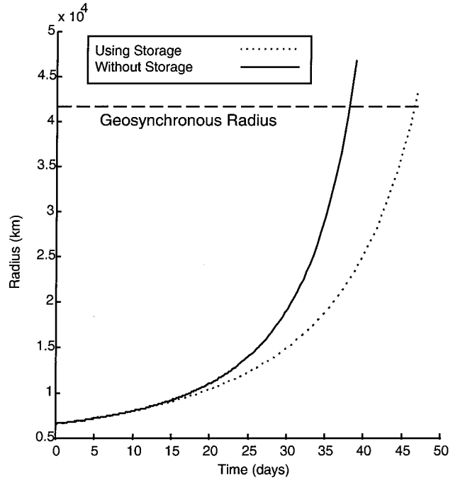
Fig. 9 Radius vs time for two spacecraft configurations.
