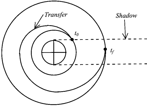
Fig. 5 Orbital-transfer segment with a low level of energy storage.
