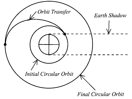
Fig. 3 Optimal circle-to-circle transfer.
