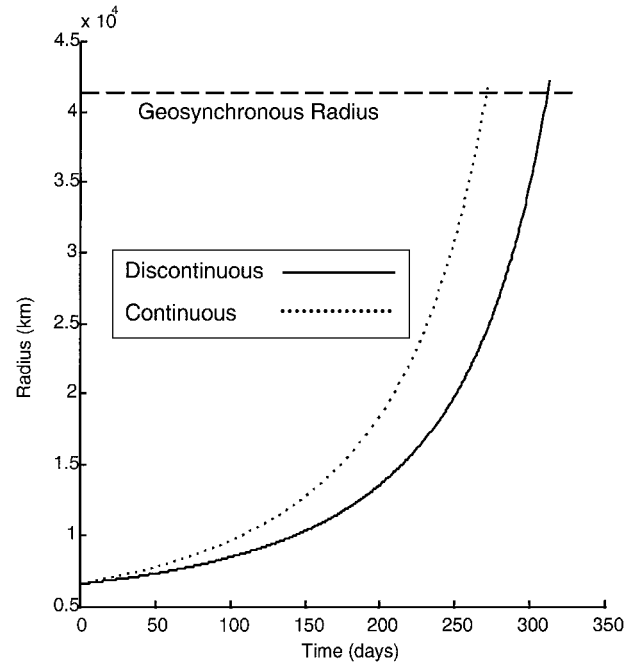
Fig. 12 Radius vs time comparison for two transfer schemes.
