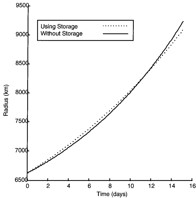
Fig. 10 Radius vs time for the first 15 days.
