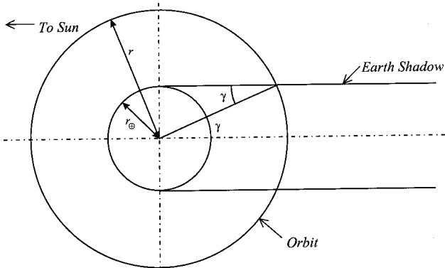
Fig. 2 Simplified shadow geometry in the ecliptic plane.
