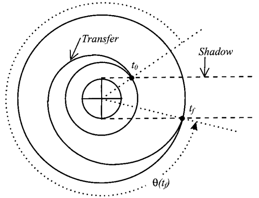
Fig. 4 Maximum transfer accomplished while in sunlight.
