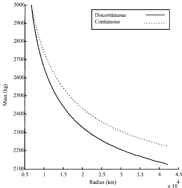
Fig. 14 Spacecraft mass vs radius comparison.
