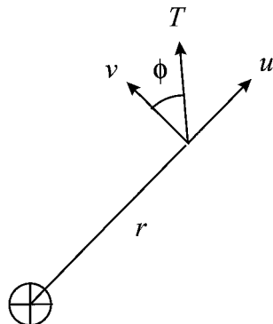
Fig. 1 Optimal transfer geometry in polar coordinates.
