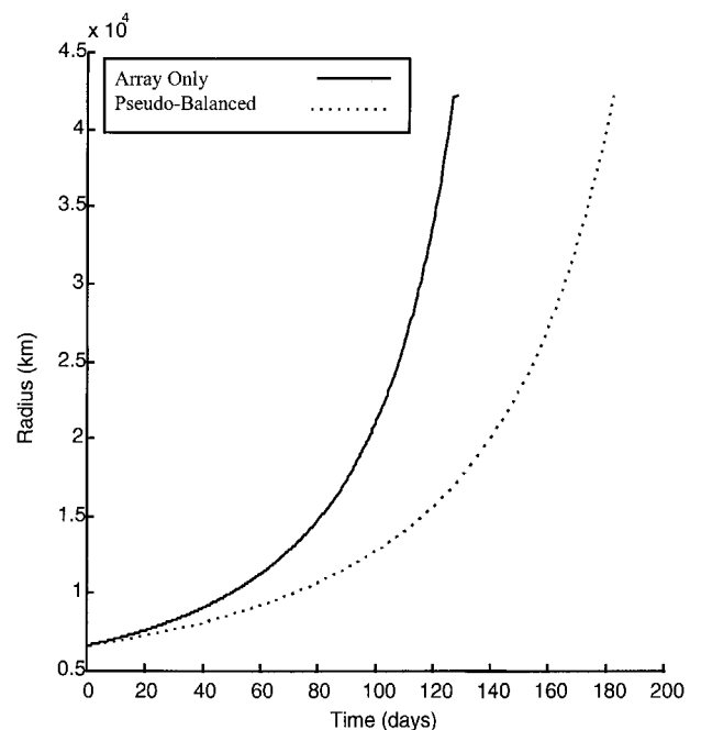
Fig. 15 Radius vs time for two extreme configurations.
