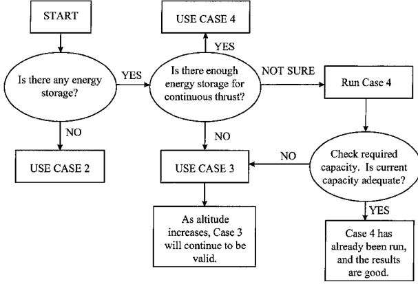
Fig. 8 Algorithm for determining appropriate case.
