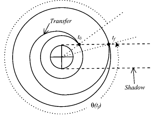
Fig. 6 Orbital transfer without a coast phase.
