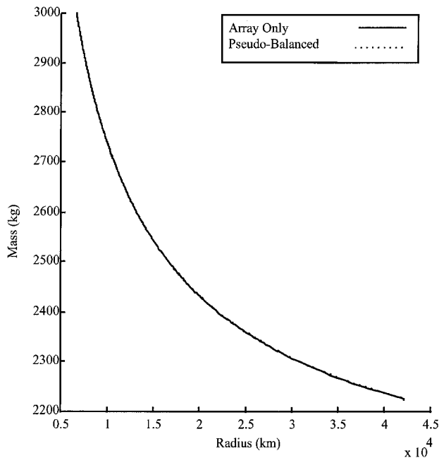
Fig. 16 Mass remaining vs radius for two extreme configurations.
