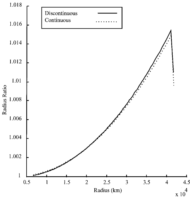
Fig. 13 Radius increase ratios vs radius comparison.
