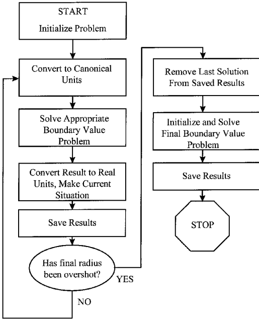
Fig. 7 Algorithm for simulating a large orbital transfer.
