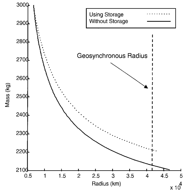
Fig. 11 Spacecraft mass remaining with respect to radius achieved.
